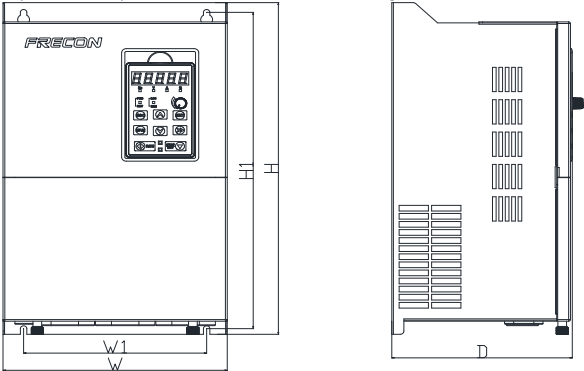
Fig 1-4 2T-18～75KW Wall installation diagram
