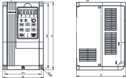
Fig 1-3 2T-4.0~11kW Wall installation diagram
