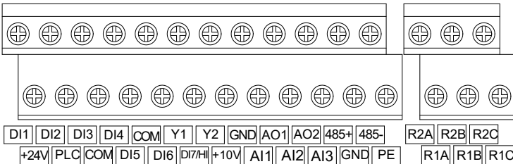
Fig.2-3b Control circuit terminals(>2.2KW)
