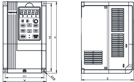
Fig 1-7 4~22kW Wall installation diagram
