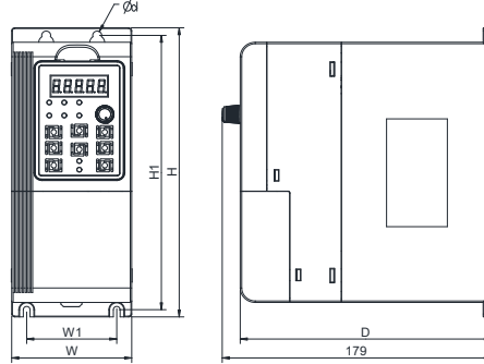
Fig 1-6 0.7~4.0kW Wall installation diagram
