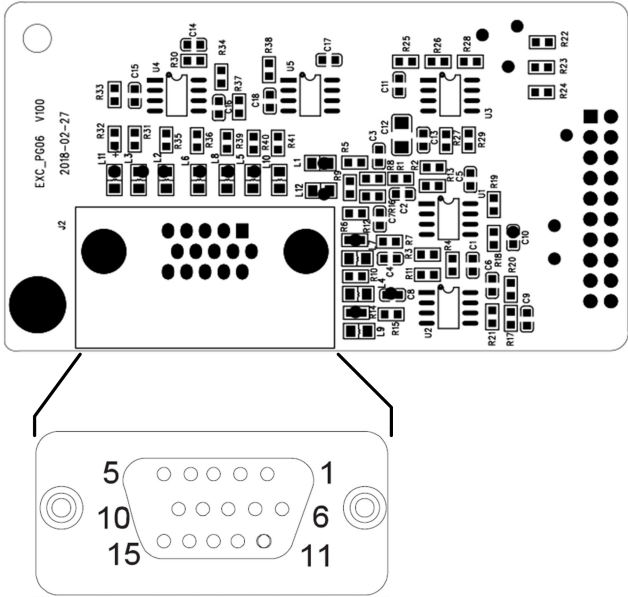
Fig.C-10 EXC-PG06 Sin-Cos encoder PG card
