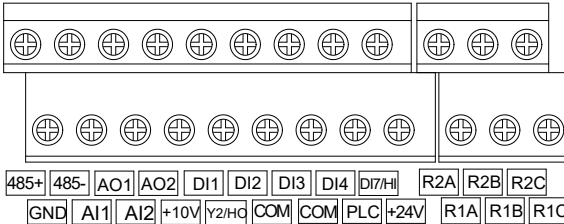
Fig.2-2a control circuit terminals (0.7~2.2kW)
